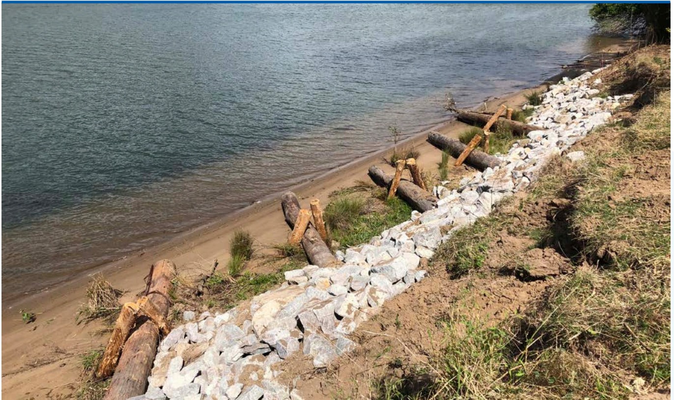
Image: Protecting the toe of the riverbank is the highest priority.
